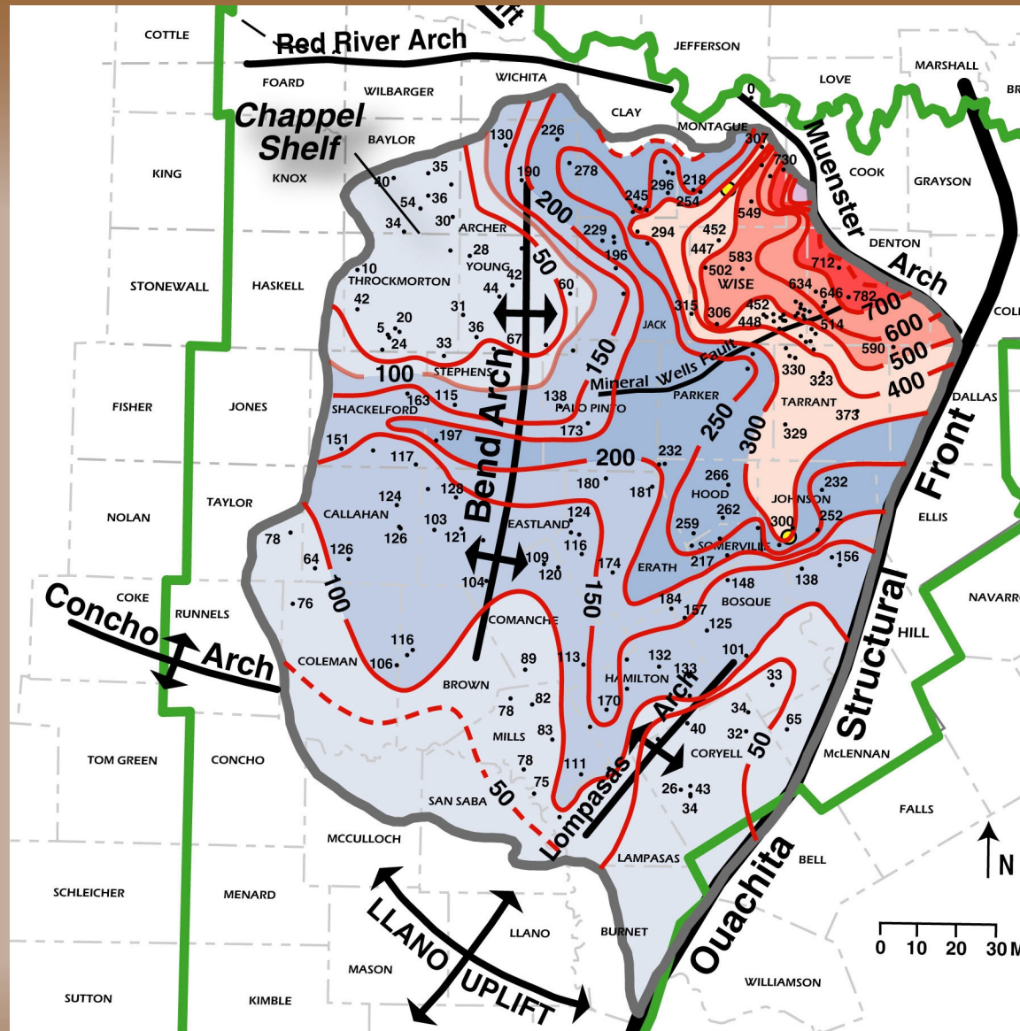
USGS Province 50 Boundary Bend Arch – Fort Worth Basin Regional isopach data, Barnett Shale – Rich Pollastro 2004
